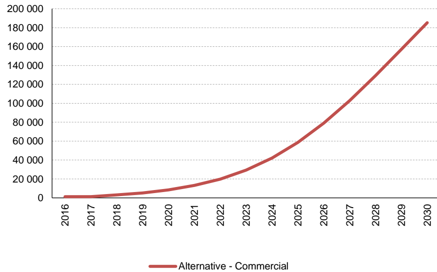
Figure 10 Evolution of Photovoltaic DG adopting commercial units between 2016 and 2030 Alternative Scenario (Commercial units)
